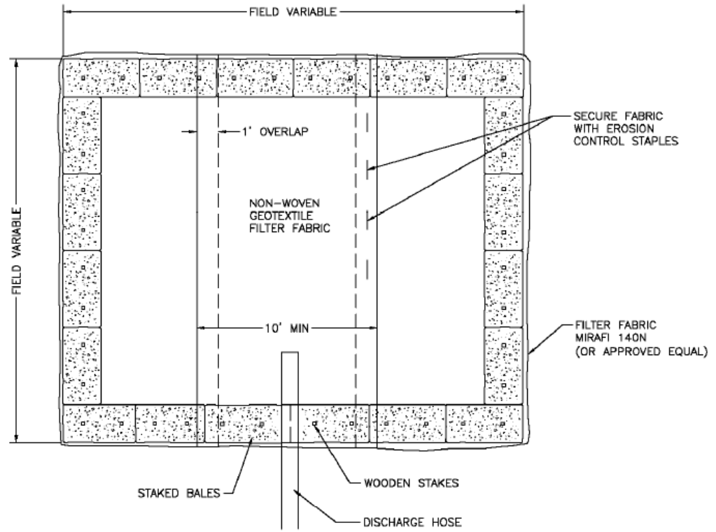
PLAN VIEW
